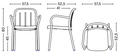
DEVILLE ARMCHAIR Width 57,5 cm Depth 52,5 cm Height 80 cm Seat height 45 cm Seat depth 41 cm Armrest height 67 cm Weight 5,4 kg
