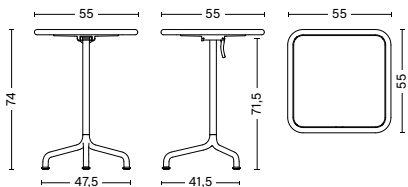
DEVILLE TABLE Width 55 cm Depth 55 cm Height 74 cm Weight 10,3 kg
