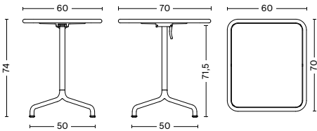
DEVILLE TABLE Width 60 cm Depth 70 cm Height 74 cm Weight 12,8 kg
