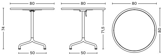
DEVILLE TABLE Diameter 80 cm Height 74 cm Weight 13,7 kg
