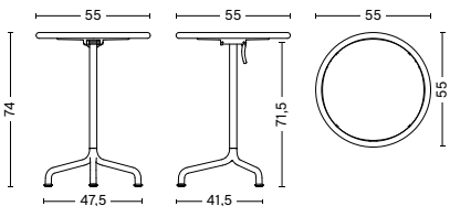
DEVILLE TABLE Diameter 55 cm Height 74 cm Weight 8,3 kg
