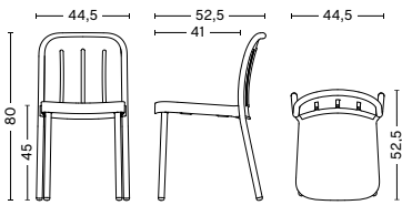
DEVILLE CHAIR Width 44,5 cm Depth 52,5 cm Height 80 cm Seat height 45 cm Seat depth 41 cm Armrest height 67 cm Weight 5 kg
